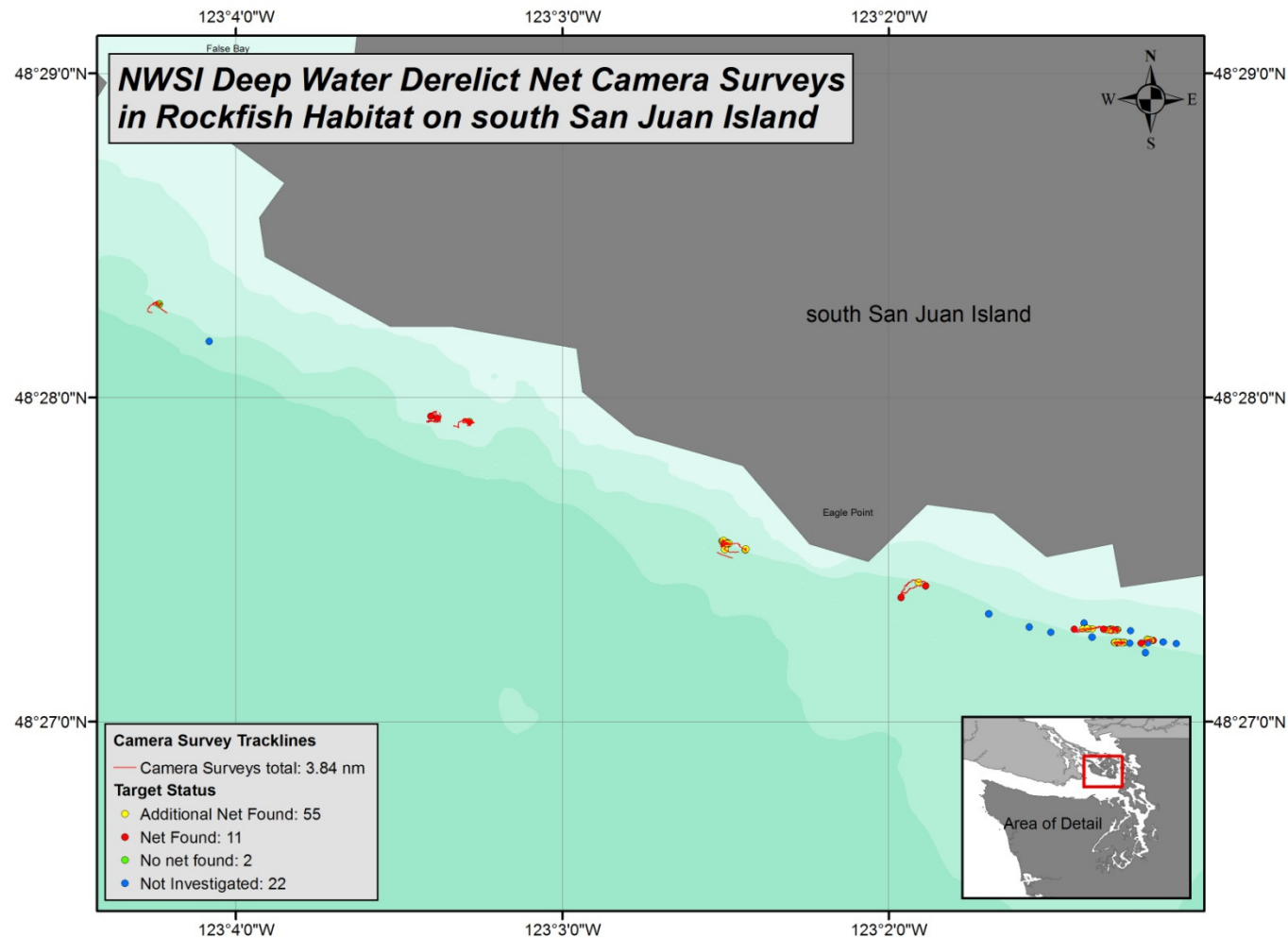
Exhibit 2: Locations and track lines of drop camera surveys of derelict fishing gear targets conducted, 2010.
